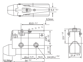
JG - XZ-7140 - Micro Switch Short Hinge Lever
