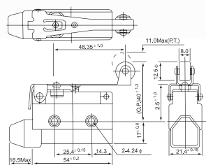
JG - XZ-7121 - Micro Switch Long Hinge Roller Lever
