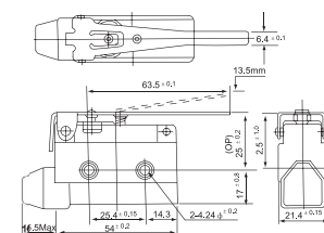
JG - XZ-7120 - Micro Switch Long Hinge Lever
