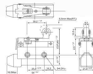
JG - XZ-7141 - Micro Switch Short Hinge Roller Lever
