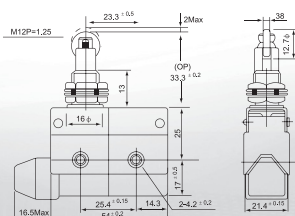
JG - XZ-7311 - Micro Switch Parallel Roller Plunger
