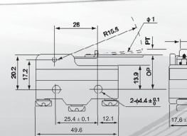
JG - XZ-15HW24-B Micro Switch Low Force Hinge Lever
