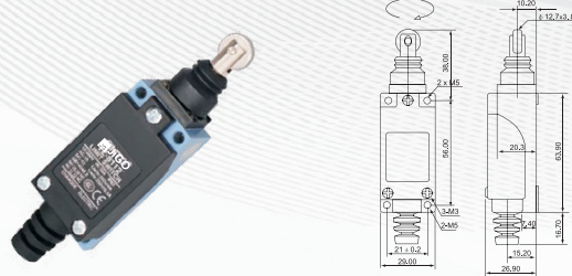
JG - XZ-8111 - Limit Switch Vertical Push Rod
